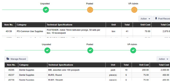
Figure 14. PR status
