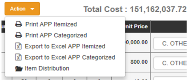
Figure 7. APP report
