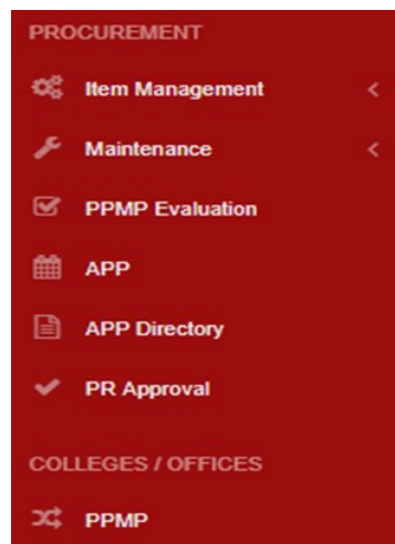
Figure 3. Procurement Module
