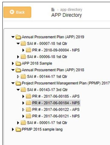
Figure 12. APP Directory
