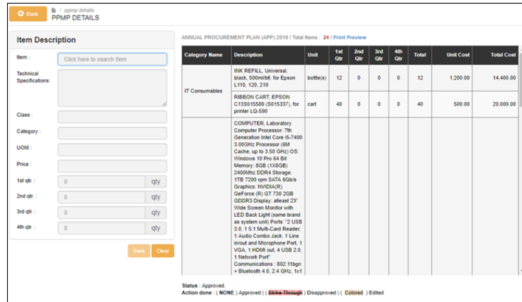
Figure 4. PPMP Details
